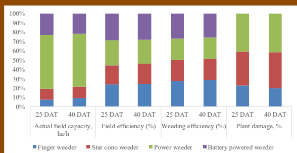
Fig. 2.21. Field performance of different weeding machine
