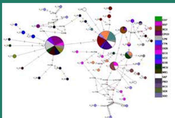
Fig. 3.9. Median joining network of mtDNA ( ITS1 ) haplotypes of BPH
