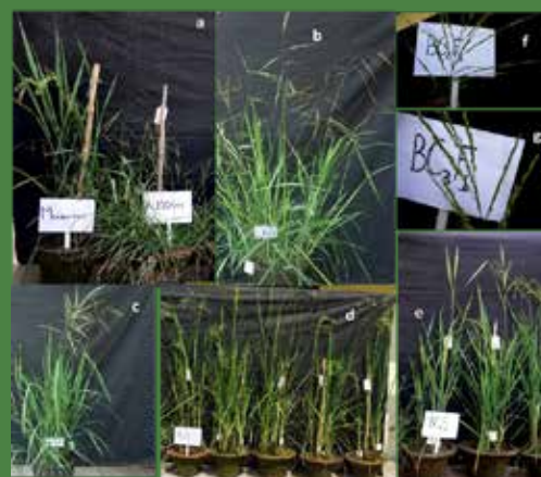
Fig. 1.3. Representative Photographs of different generations of Maudamani and O. rufipogon (AC 100444) cross. a. parental lines; b. F_1 plants; c. BC_1F_1 plants; d. BC_2F_1 plants; e. BC_3F_1 plants; f. representative panicle of BC_2F_1 plants and g. representative panicle of BC_3F_1 plants
