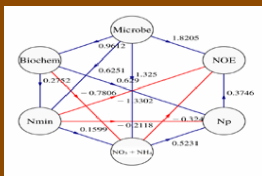
Fig. 2.5. PLS (partial least square) model of different parameters at elevated \text{CO}_2 ( 550 \pm 20 \mu\text{mol mol}^{-1} ). Microbes represented by the variables like population of soil nitrifiers and denitrifiers and soil biochem represented by variables like FDA = fluorescein diacetate, \beta -glucosidase and urease. \text{N}_{\min} = nitrogen mineralization, \text{NO}_3^- \text{N} = nitrate nitrogen, \text{NH}_4^+ \text{-N} = ammonical nitrogen, Np = nitrification potential, NOE = nitrous oxide emission. Lines with blue colour represent positive relation, whereas red colour represents negative relation. The numbers represent coefficient values.
