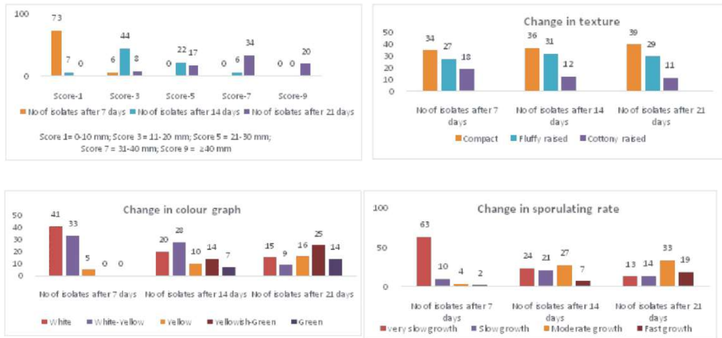
Fig. 1. Morphometric variation of isolates of U. virens collected from eastern and north-eastern India.
